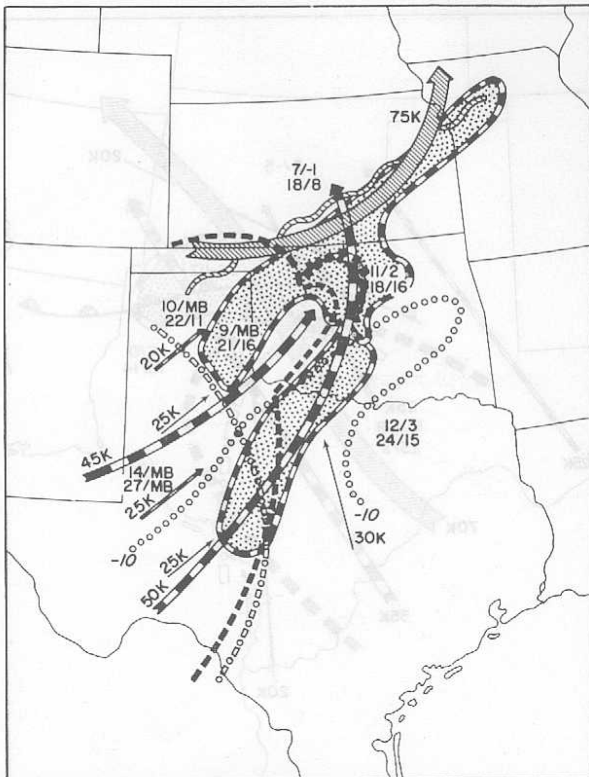
Figure 19. Significant upper-air features including Oklahoma State University radar echoes. Echoes at 0210Z are a line of solid circles and the echoes at 0345Z are a line of solid squares. Stippled area outlines locations of severe-weather occurrences.
