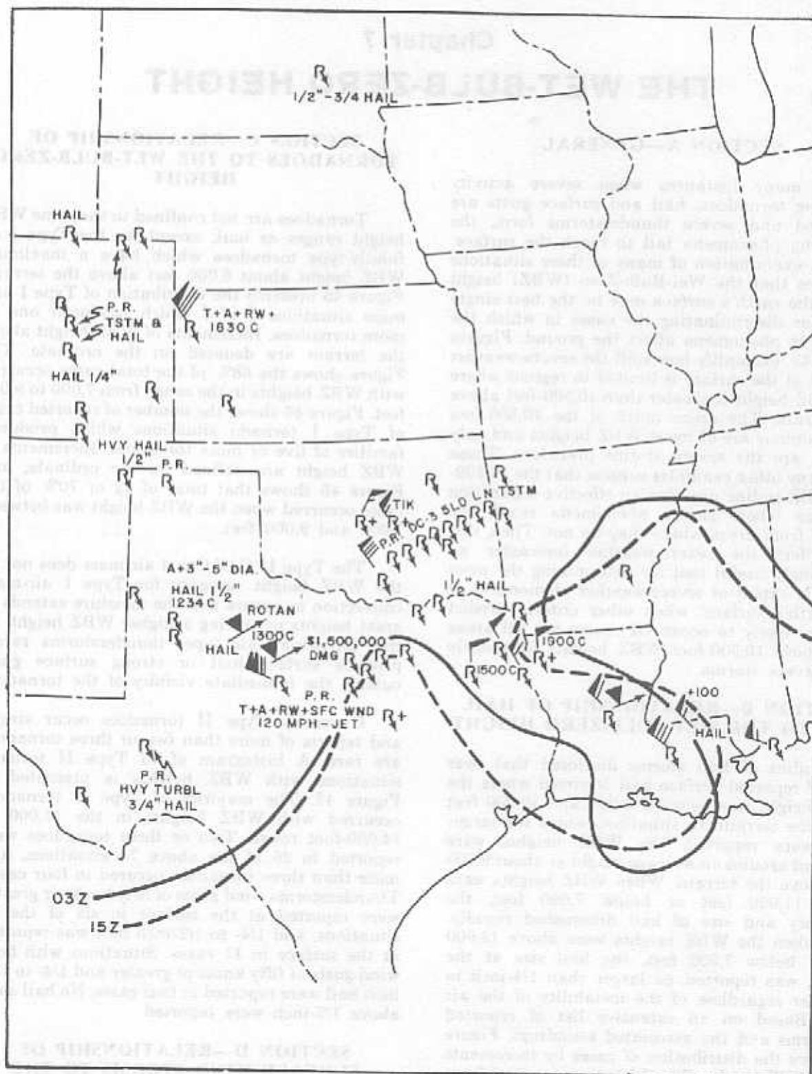
Figure 41. Location of 10,500-foot Wet-Bulb-Zero isopleth and areas of severe-weather activity from 1500Z 10 June to 0300Z 11 June 1951
