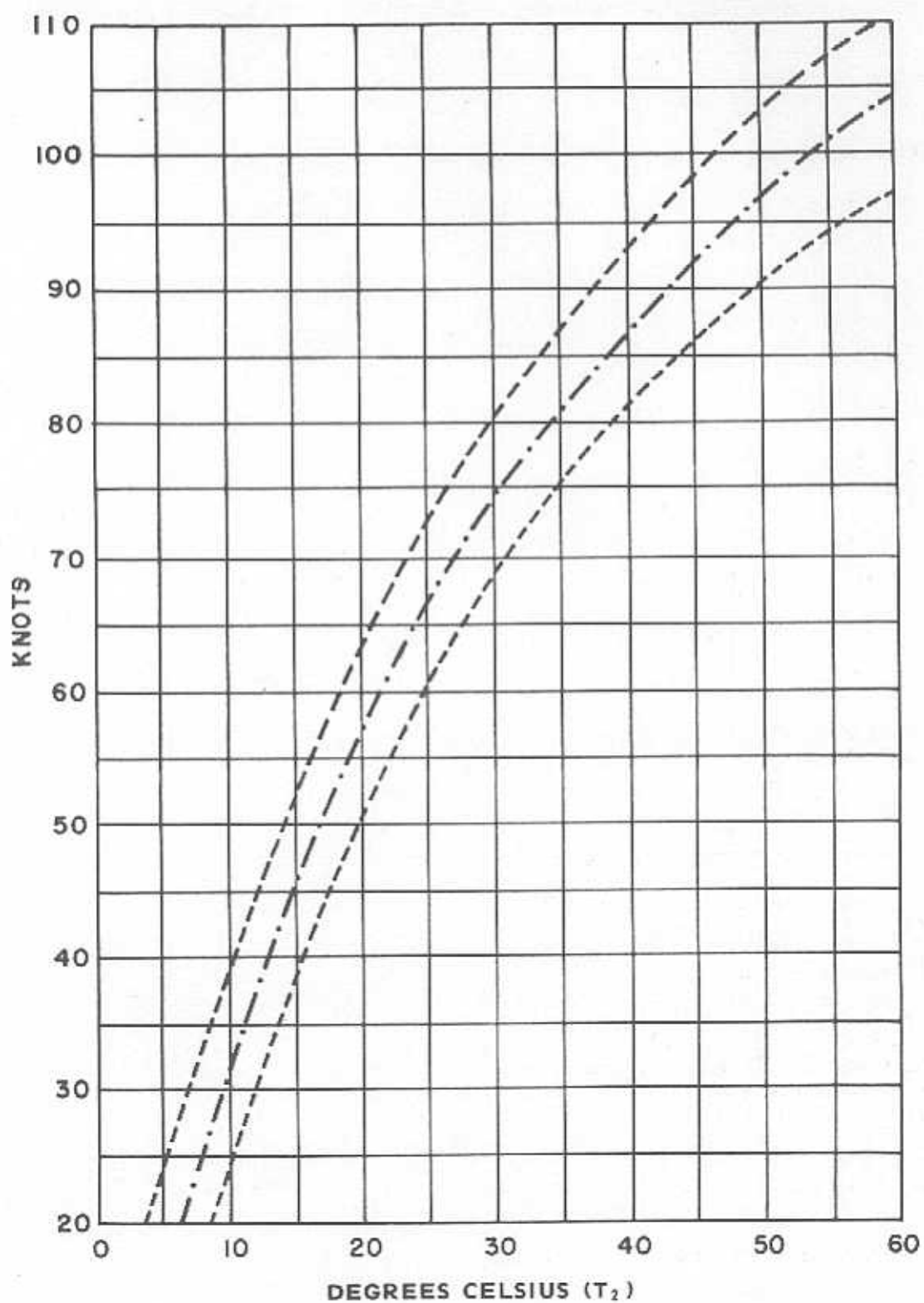
Figure 53. Alternative gust forecasting technique. Useful in the Type II air mass.
