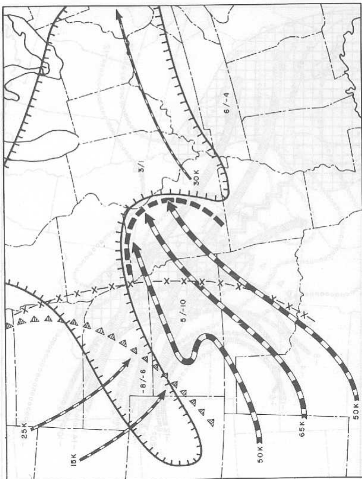
Figure 60. Major Features of the 700-mb chart at 1200Z 26 November 1965.
