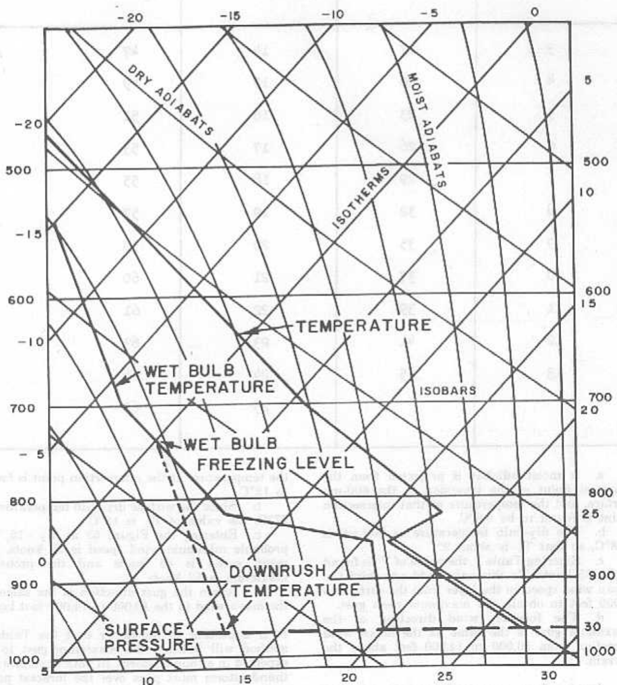
Figure 52. Determination of downrush temperature by tracing a saturation adiabat from intersection of wet bulb curve and 0°C isotherm to the surface pressure.
