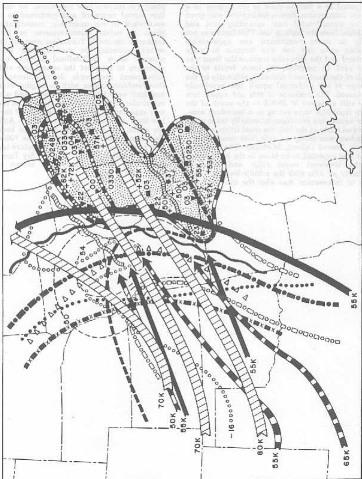
Figure 63. Composite Chart of the 1200Z 26 November 1965 data. Includes the severe activity during period 260000Z to 261200Z.
