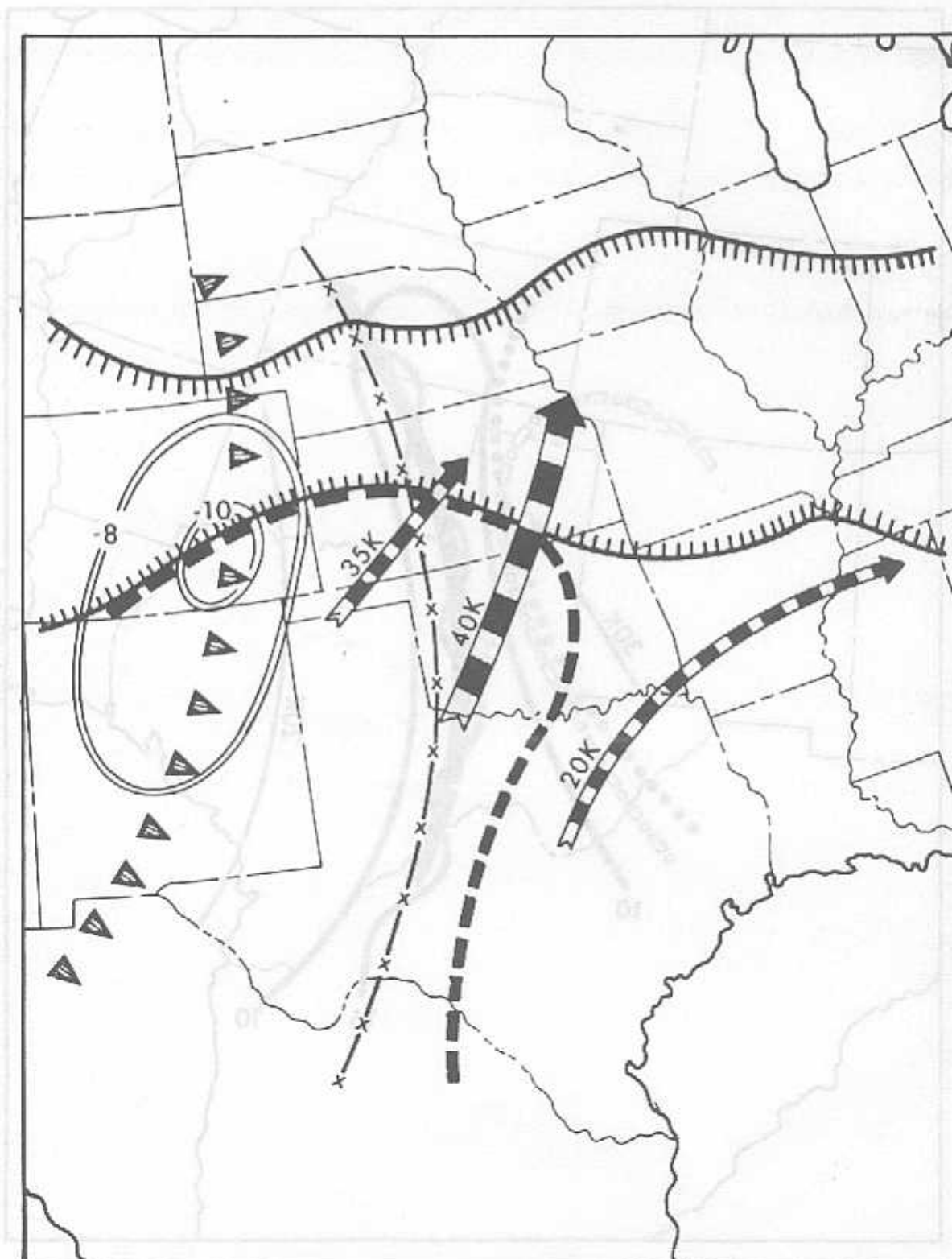
Figure 66. Major features on 700-mb chart for 08/1700Z.
