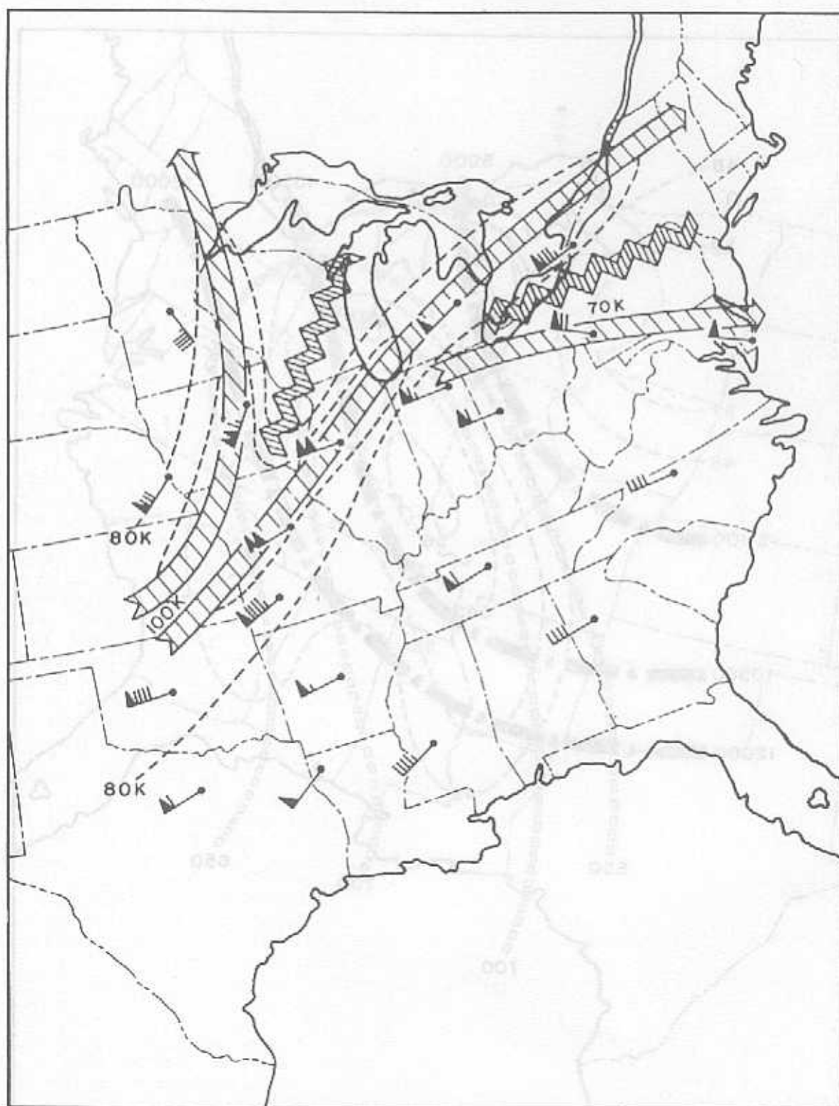
Figure 31. An example of the Maximum-Wind Chart for the Palm Sunday tornadoes of 11 April 1965
