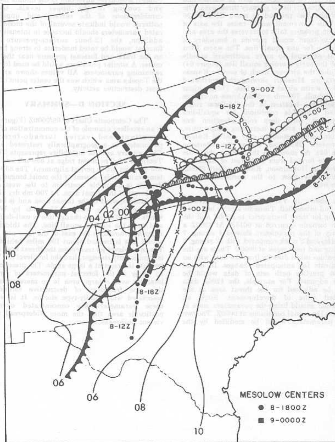
Figure 64. Location of major surface features during period 08/1200Z to 09/0000Z. Isobar analysis is for 08/1200Z.
