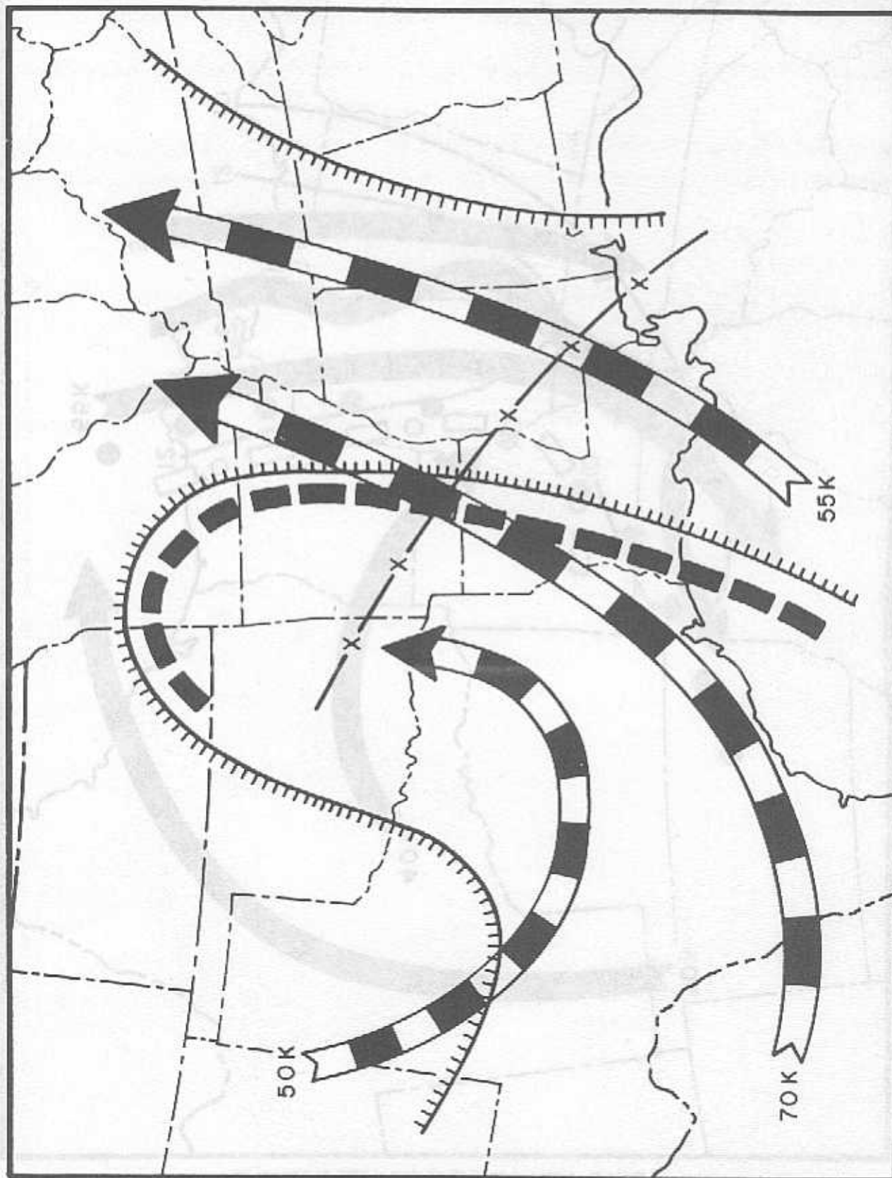
Figure 88. Major features of 700-mb chart at 0600Z, 22 February 1971.
