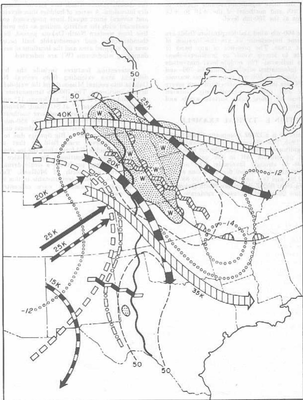
Figure 40. Composite Chart for 1200Z 26 August 1965 is a typical summertime severe-weather pattern
