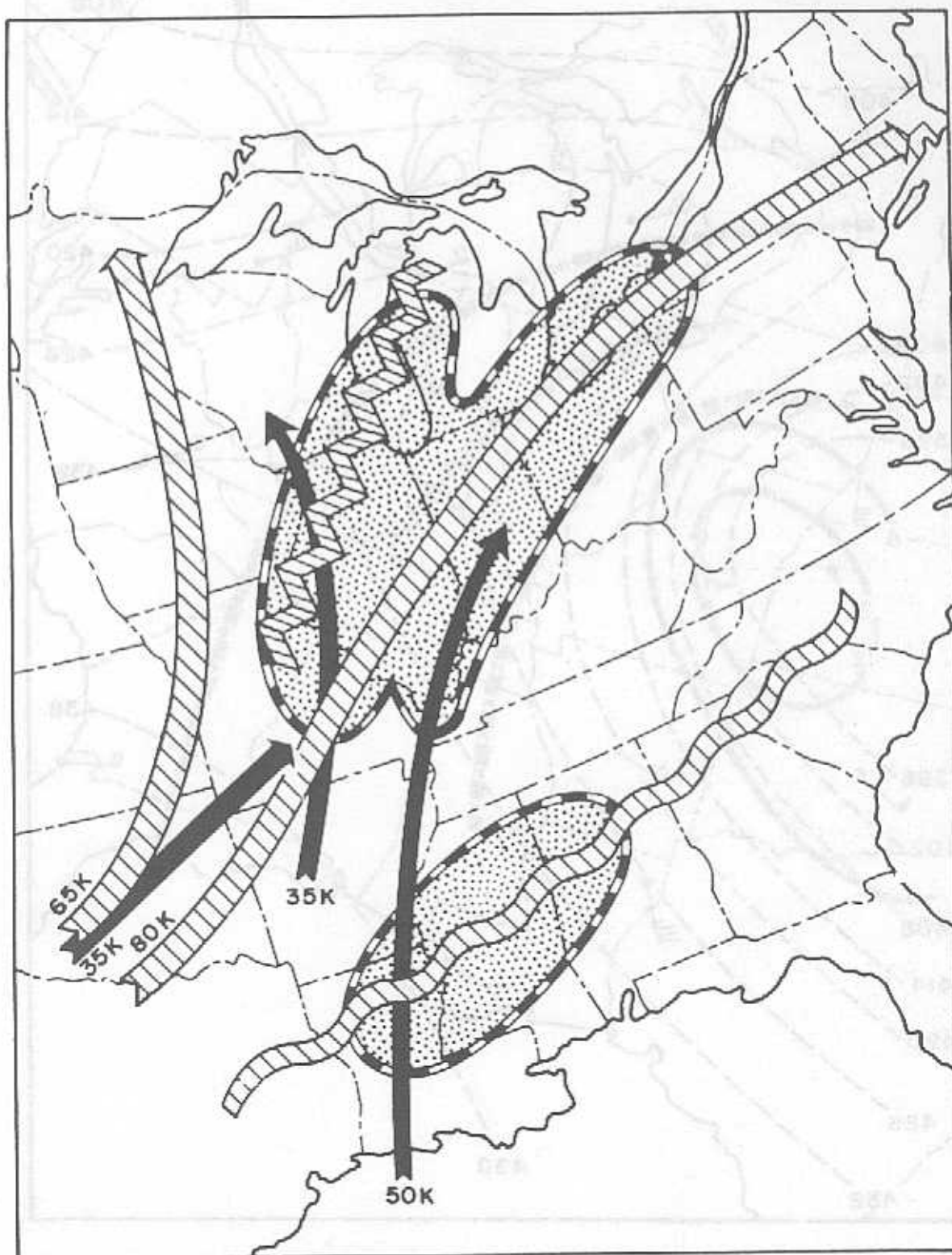
Figure 37. Example of low- and higher-level wind fields. Stippled areas outline regions of severe-weather occurrences.
