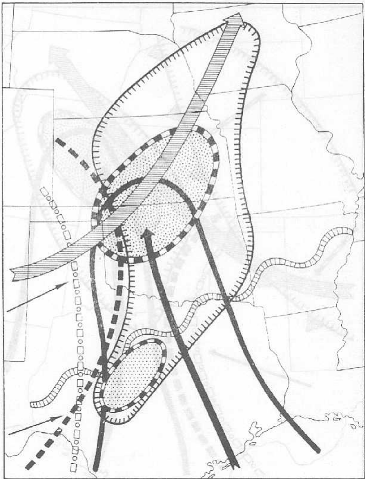
Figure 12. The Type A tornado-producing synoptic pattern. Stippled area outlines location of severe-weather occurrences.
