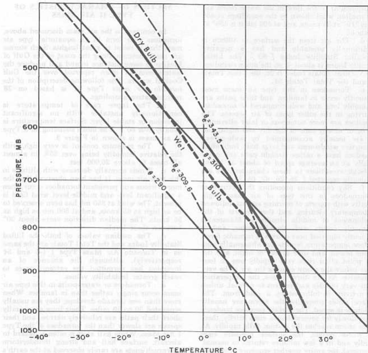
Figure 9. Mean Sounding of Type II Tornado Air Mass
