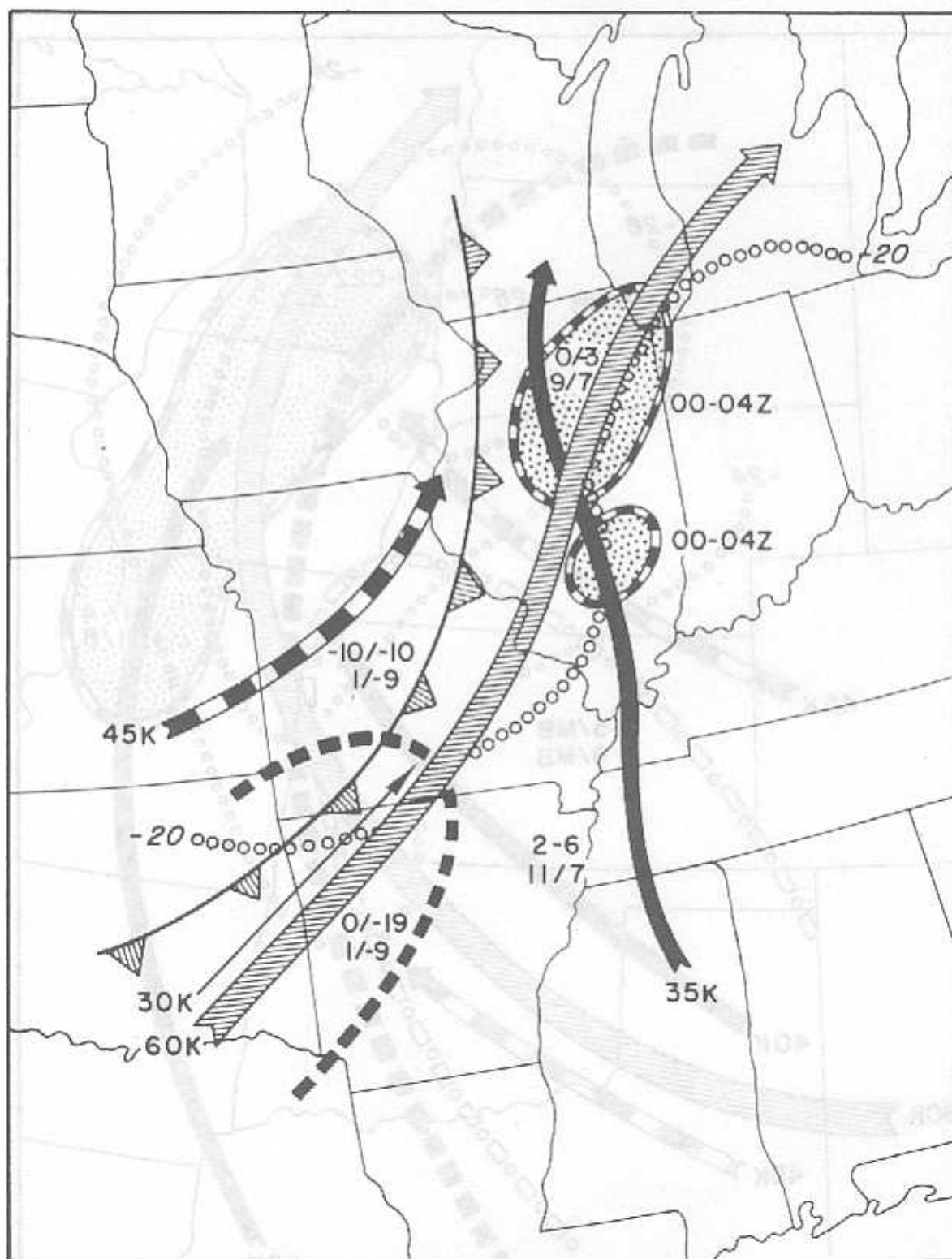
Figure 24. Example of Type E pattern showing significant features at 2100Z on 14 March 1957. Stippled area outlines locations of severe-weather occurrences.
