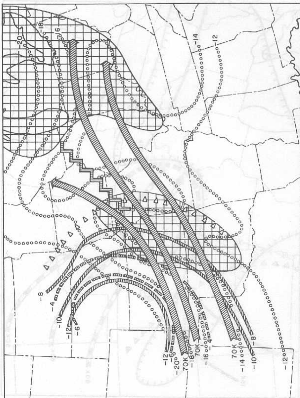
Figure 61. Major features of the 500-mb chart at 1200Z 26 November 1965.
