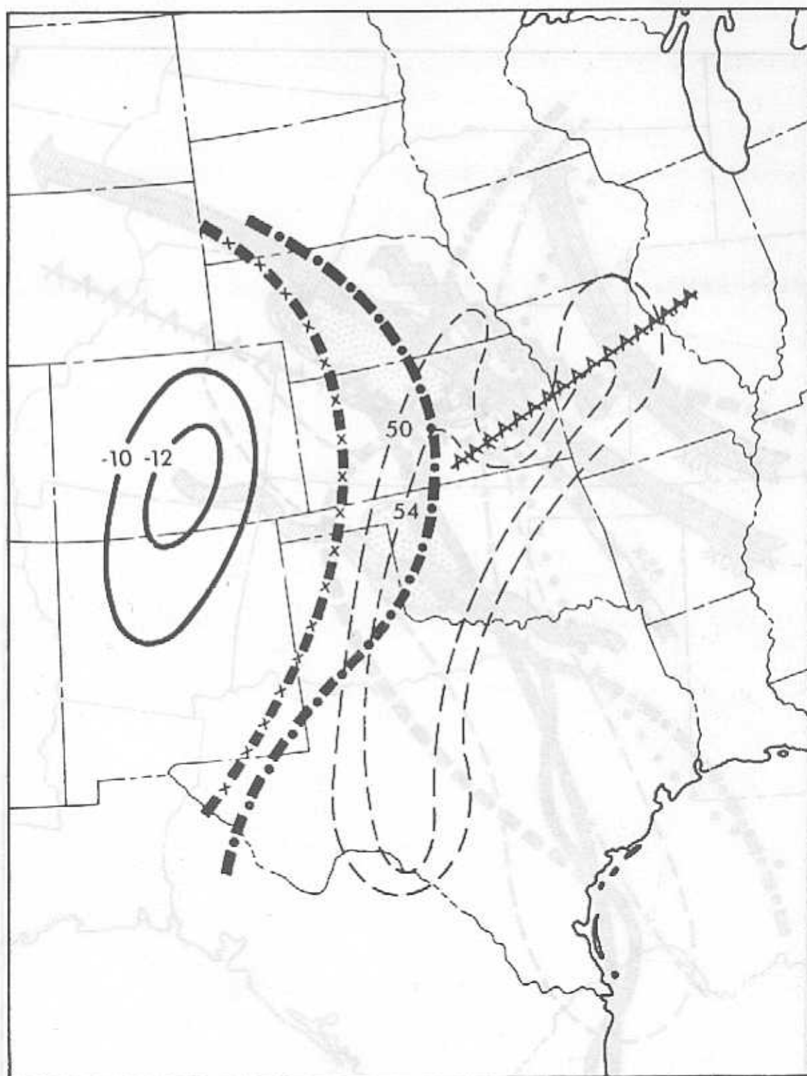
Figure 69. Thickness change, no-change line, thickness ridge line, and Total Totals at 06/1200Z. Also shows zone of anti-cyclonic wind shear.
