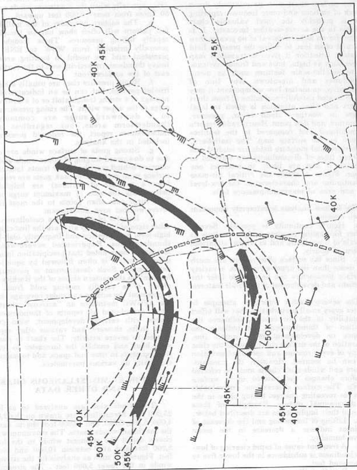
Figure 5. Maximum wind analysis for the lower 5,000 feet
