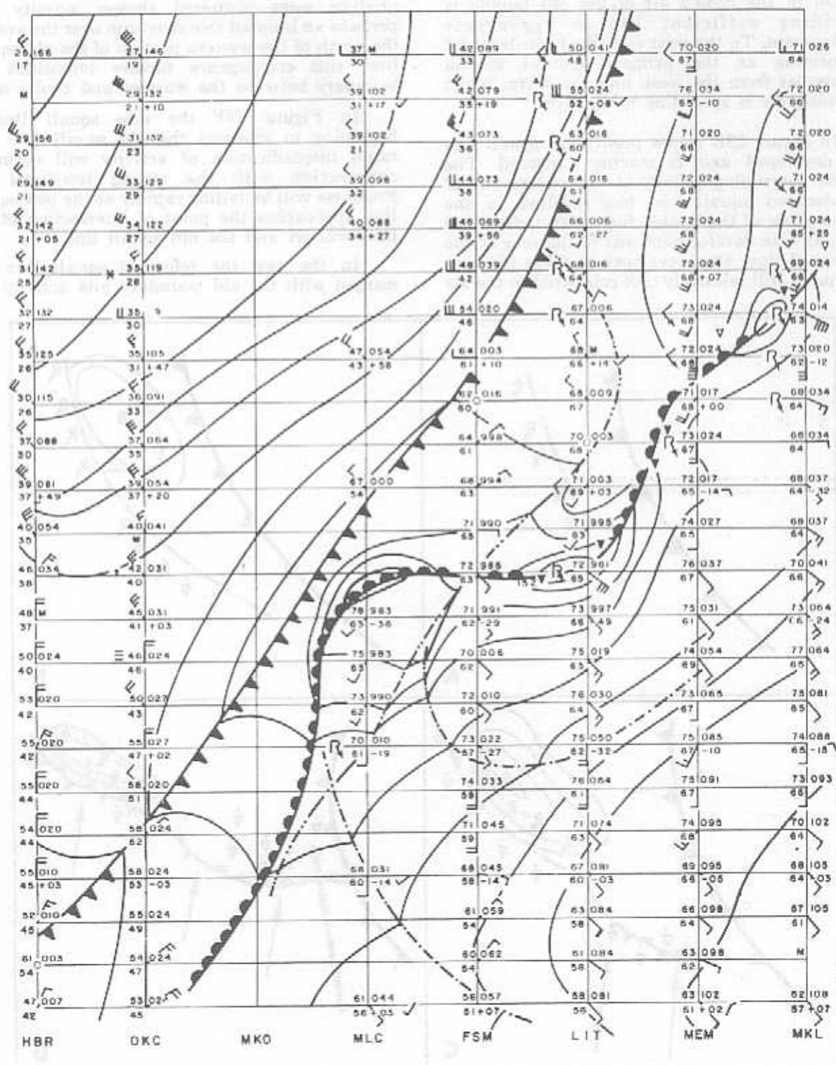
Figure 27. Time cross-section of development and movement of mesolows and accompanying tornadoes of 22 March 1952.
