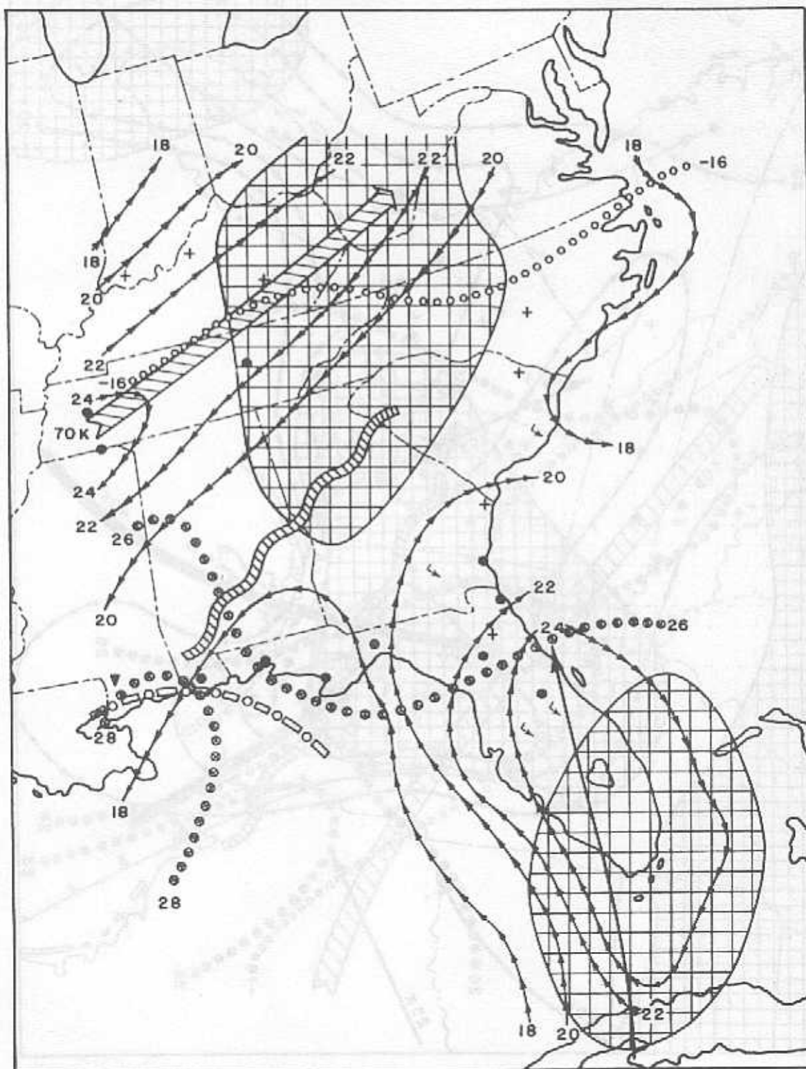
Figure 56. Composite chart for 1200Z 3 December 1964 showing parameters of interest and activity during period 031200Z to 040000Z
