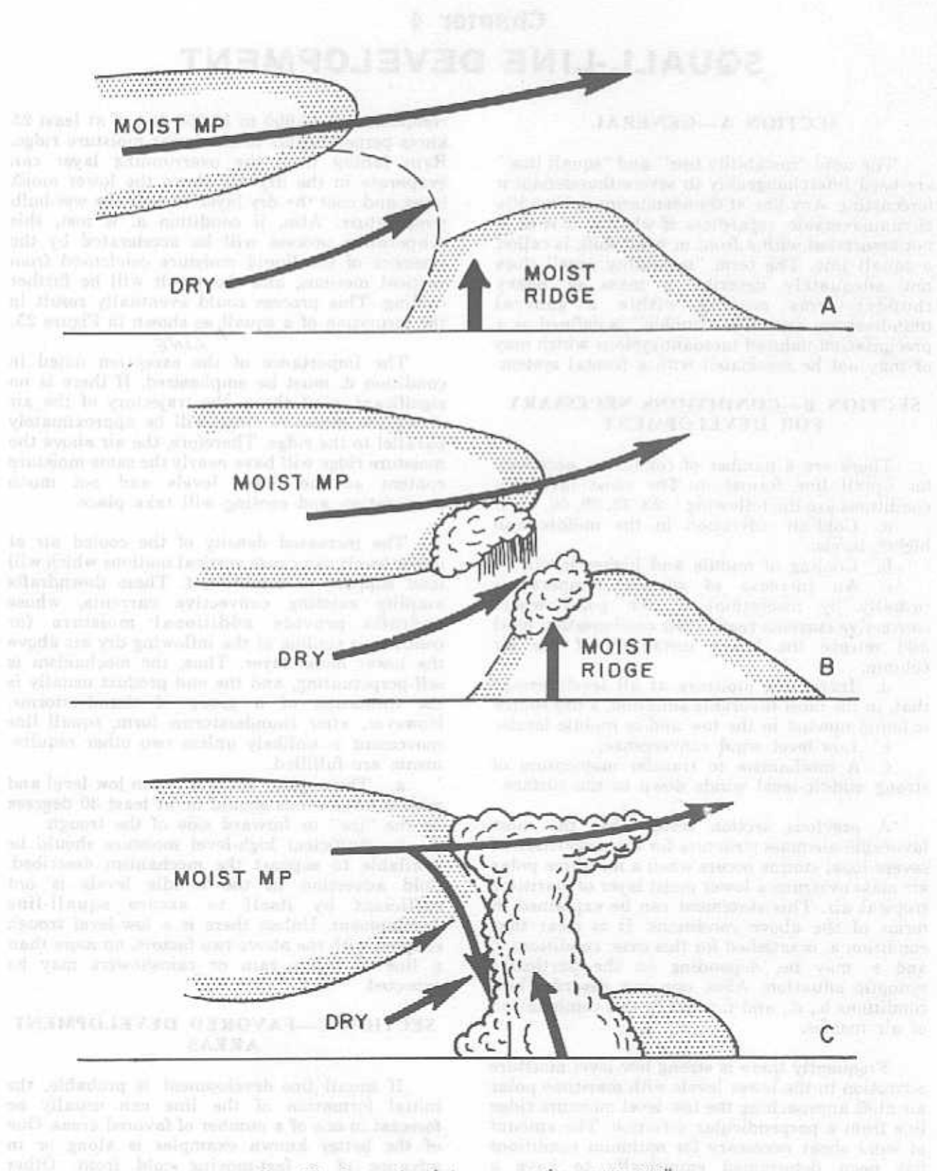
Figure 25. Cross-section of air mass suggesting one way squall lines can develop.
