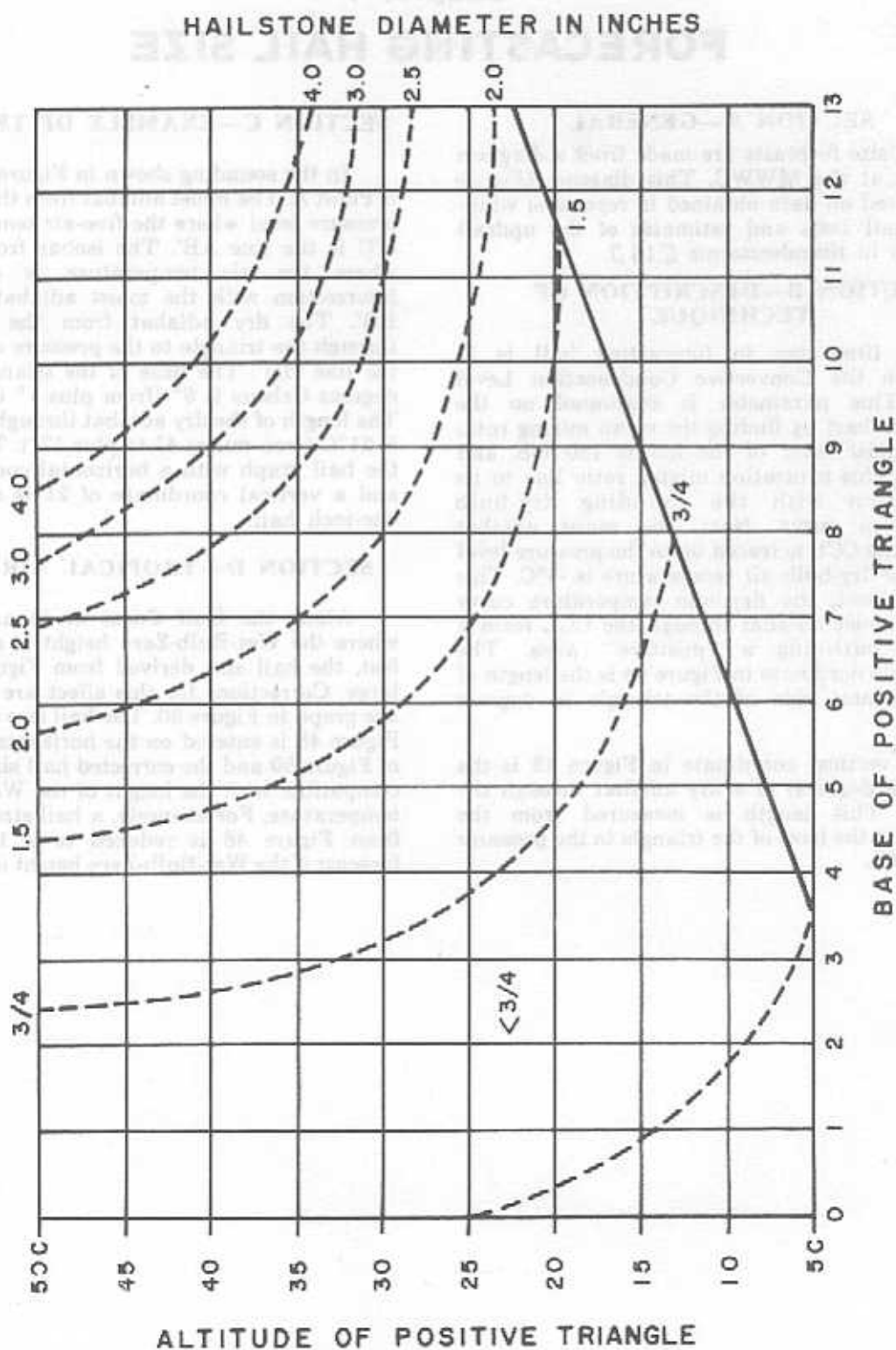
Figure 48. The Fawbush-Miller Hail Graph showing the forecast hailstone diameter in inches. Graph revised November 1965 on the basis of 622 hail reports.
