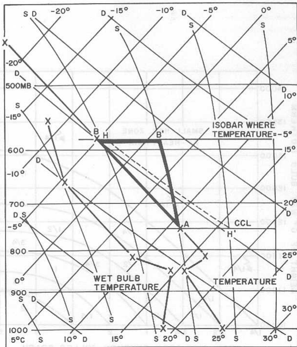
Figure 49. Example of hail size forecast from sounding. BB' is the base of the positive triangle and HH' measures the altitude. In this case 6 and 21 respectively. These values are equivalent to one-inch hailstones in Figure 45.
