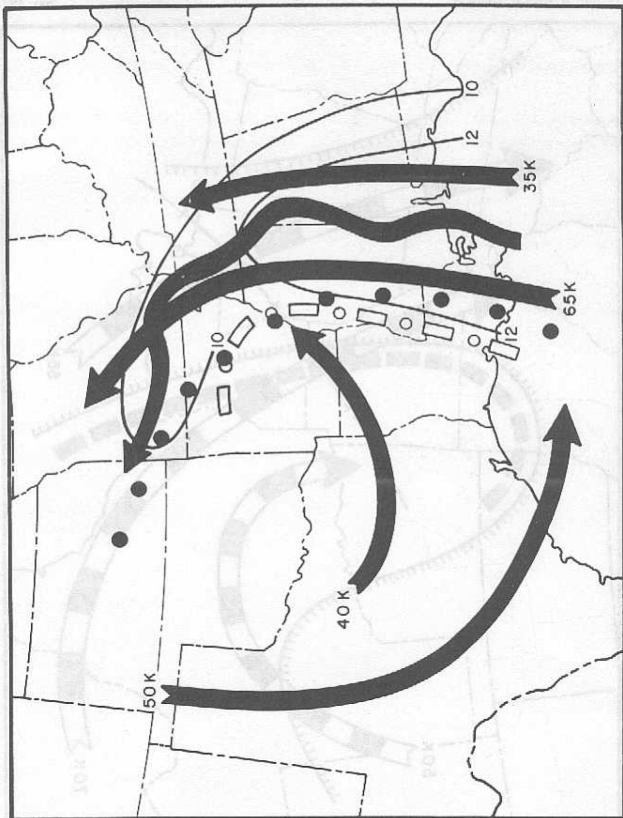
Figure 37. Major features of 850-mb chart at 0000Z, 22 February 1971.
