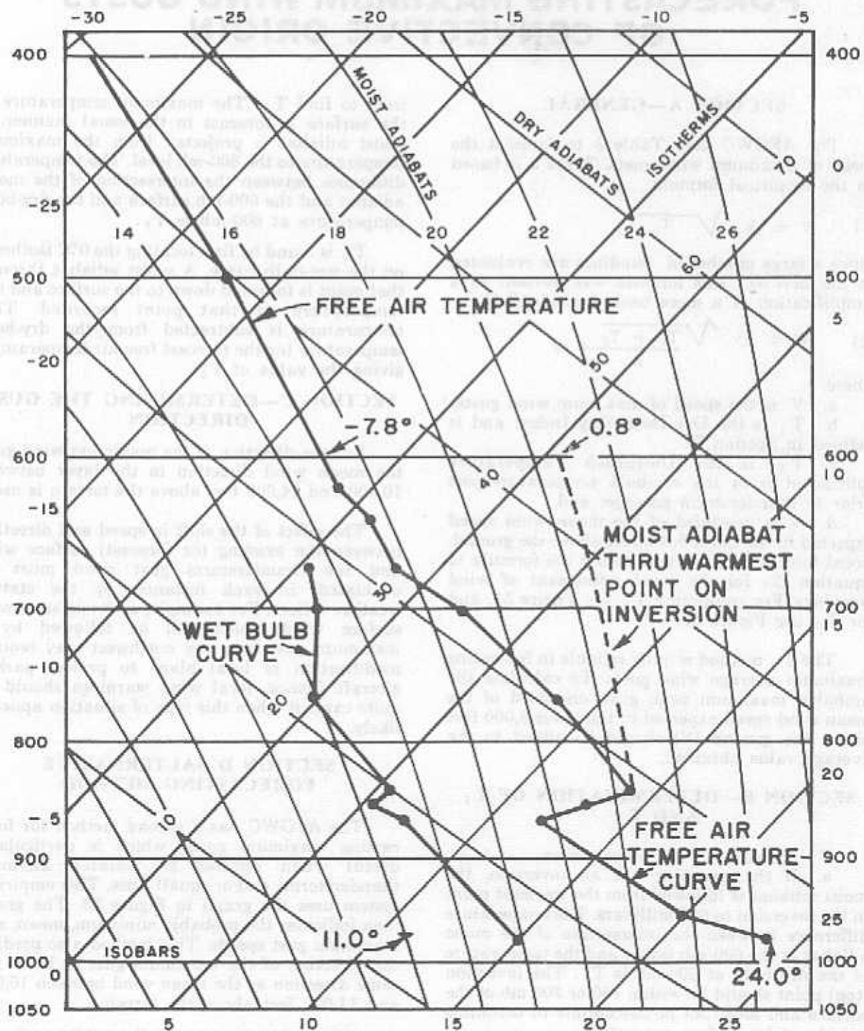
Figure 51. Example of sounding for wind gust forecast.
