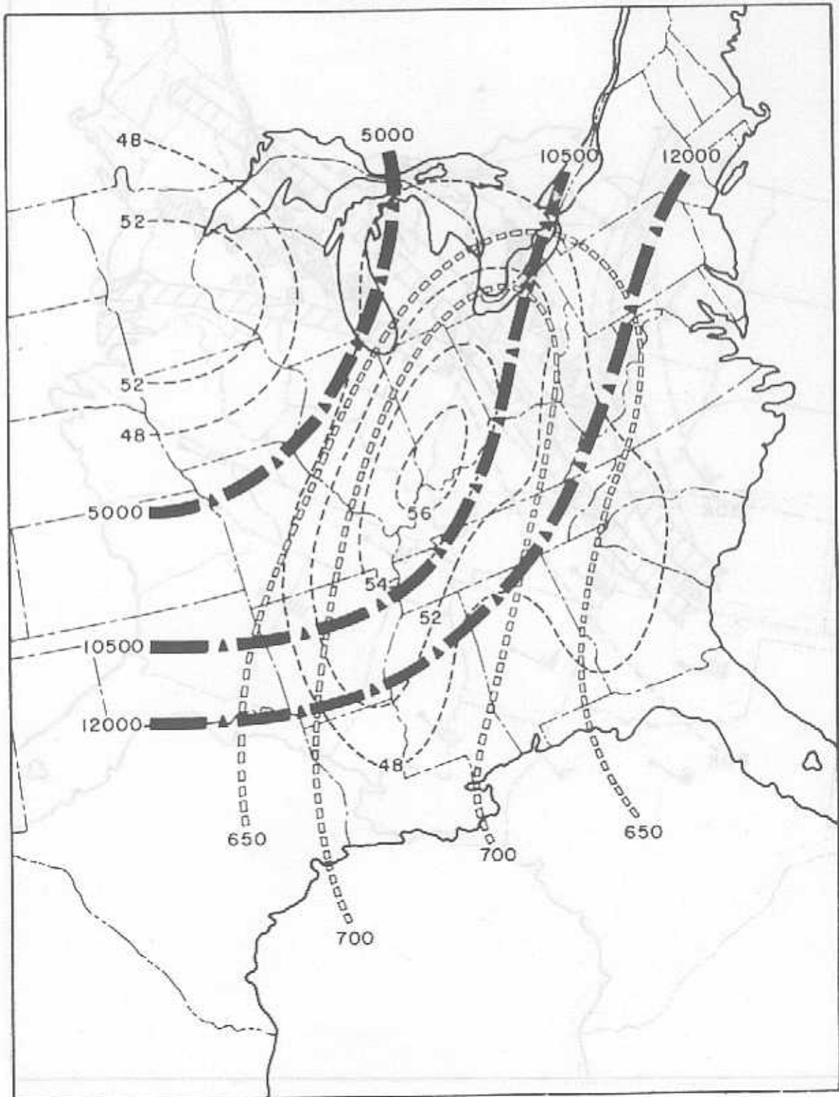
Figure 30. Stability analysis showing Total Totals and Lifted Indexes. Also, isopleths of the height of the Wet-Bulb-Zero and LFC are indicated.
