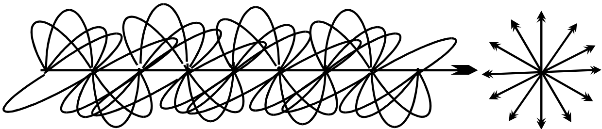
Ordinary Light Waves
