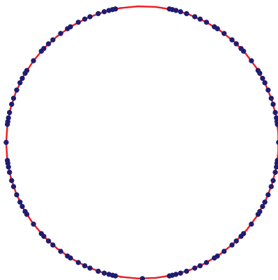
FIGURE 4. 111 points along \mathbb{RP}^1 .
