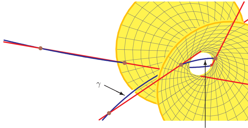
FIGURE 3. The problem of four secant lines.
