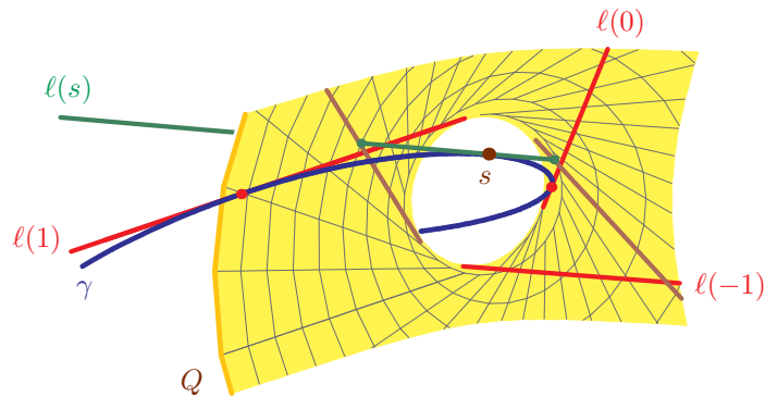
FIGURE 2. Configuration in the throat of the quadric.
