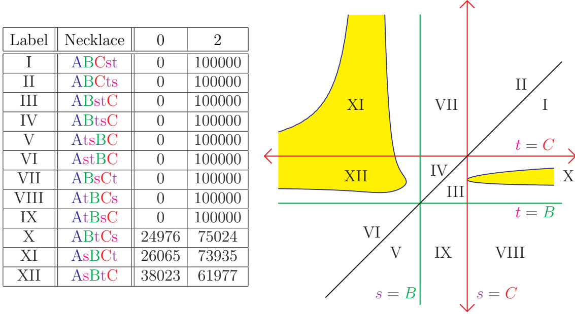
FIGURE 6. The Schubert problem (\sigma_1, 4\ 3\ 1256, 13\ 25\ 46, 1256\ 4\ 3, \sigma_5) on \mathbb{F}l(1, 2, 4, 5; 6) and its discriminant.
